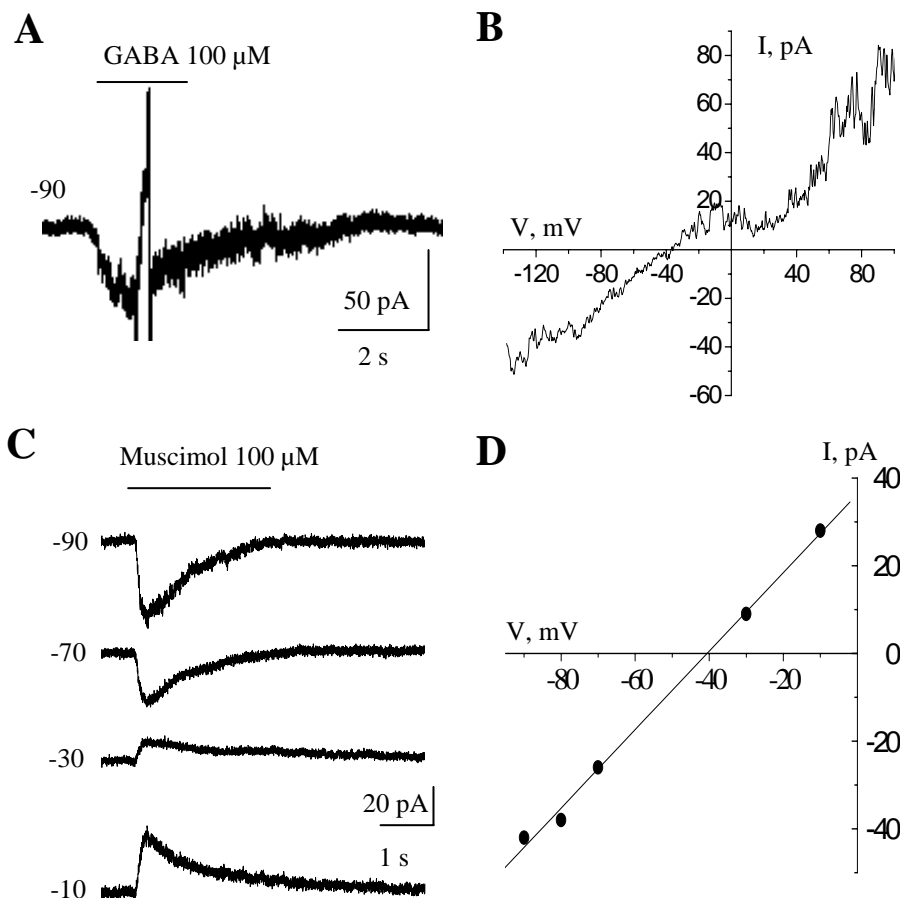
Figure 6. Estimation of intracellular [Cl^-] using GABA_A responses and gramicidin perforated patch-clamp recordings of Bergmann glia. A. 100 \mu M GABA-induced current with the gramicidin perforated patch-clamp technique. A ramp protocol was applied near the peak of the current. B. I-V curve of the GABA response shown in (A). C. Muscimol-induced currents recorded at different holding potentials. Recordings were obtained with the perforated patch-clamp technique. D. I-V curve of the muscimol responses shown in (C).
